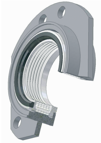
Single Seal Arrangement
